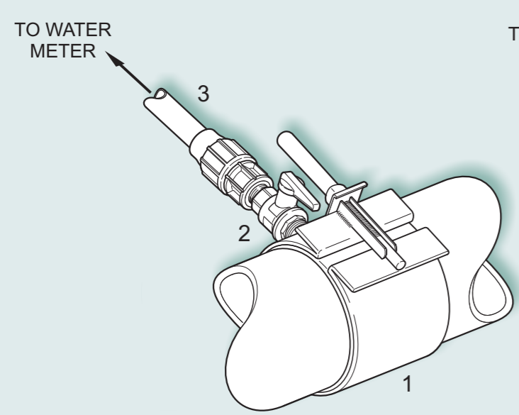
TAPPING UNDER PRESSURE UP TO 50mm (BALL VALVE)
