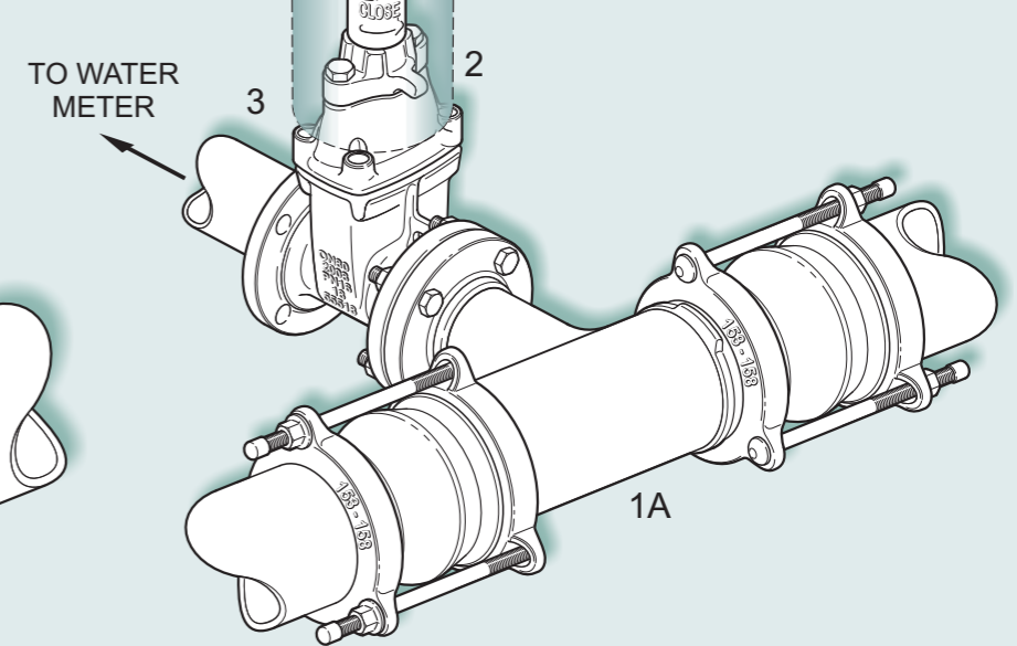
TEE INSERTION GREATER THAN 50mm (MAIN SHUT DOWN)
