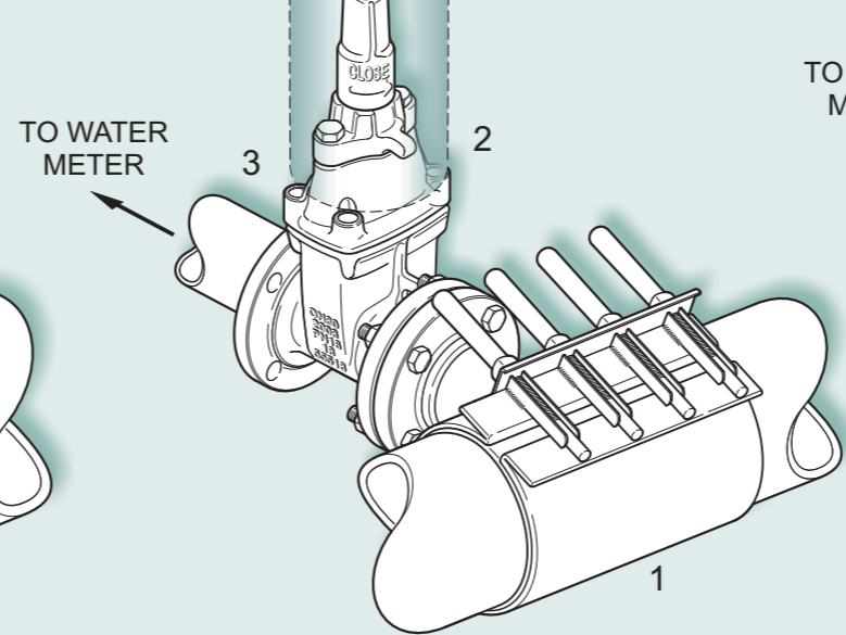
TAPPING UNDER PRESSURE GREATER THAN 50mm
