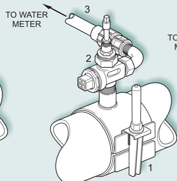
TAPPING UNDER PRESSURE UP TO 50mm (FERRULE & BEND)
